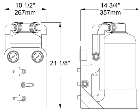
MULTI-MEDIA FILTER
