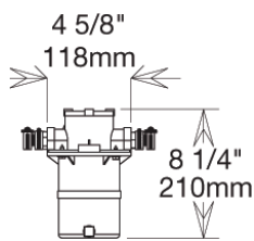
Sea Strainer
