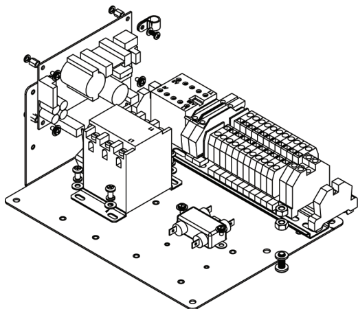
Electrical Chassis-Single Phase
