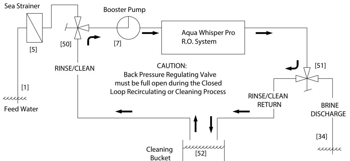
Figure 6: Simplified Aqua Whisper Pro RO Desalination System Recirculating Loop
