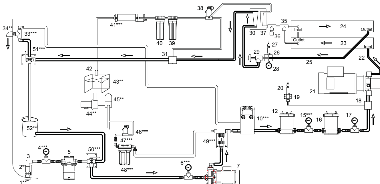
Figure 3: Aqua Whisper Pro RO Desalination System Illustrated in a Once Through Configuration for Flushing the System with Fresh Water and for discharging Cleaning or Storage Chemical (with Inlet Rinse / Clean Valve or the Outlet Rinse / Clean Valve)
